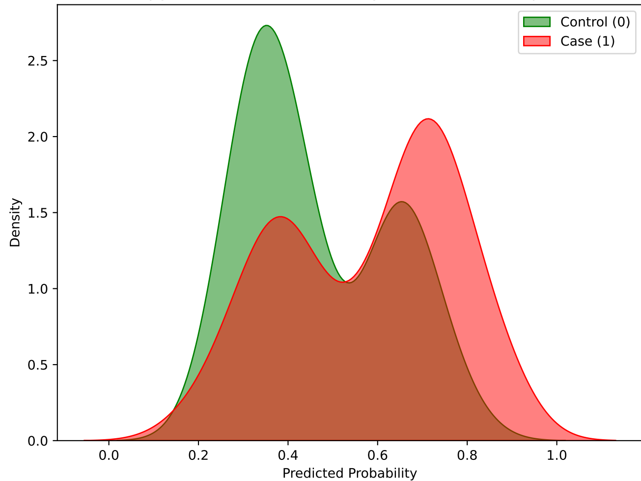
Polygenic Risk Score (Probability) Distribution - DeepRisk
